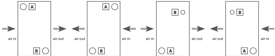
Fig. 4a. Fluid flow direction in respect of air flow in collers with rectangular connetions A – water/refrigerant out, B – water/refrigerant in
